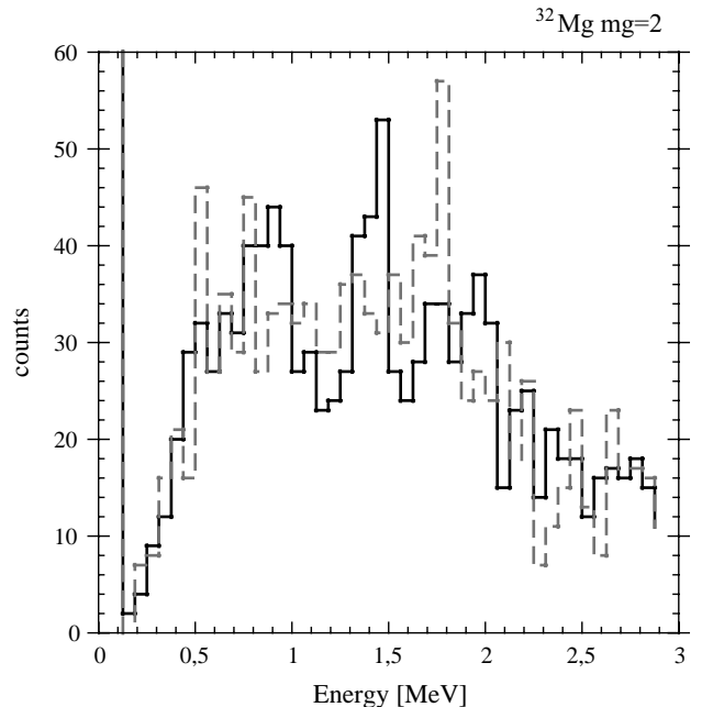
Fig. 2. Experimental \gamma -spectra for multiplicity m = 2 for inelastic scattering of ^{32}\text{Mg} . Full and broken lines correspond to the spectra after and before Doppler correction. In the uncorrected spectrum the 1.78 MeV line of ^{28}\text{Si} shows up, in the Doppler-corrected spectrum one can see the 1.4 MeV and 0.88 MeV transitions.
