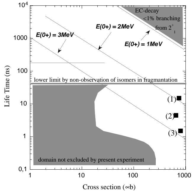
Fig. 1. Lifetime and inelastic scattering correlation for a monopole transition in ^{34}\text{Si} . Lines are labelled for different excitation energies of the 0^+ state. The lower limits obtained in the present experiment are given by the shaded area. The squares marked 1, 2, 3 correspond to values expected in the models of [16, 18, 13], respectively (see text).
